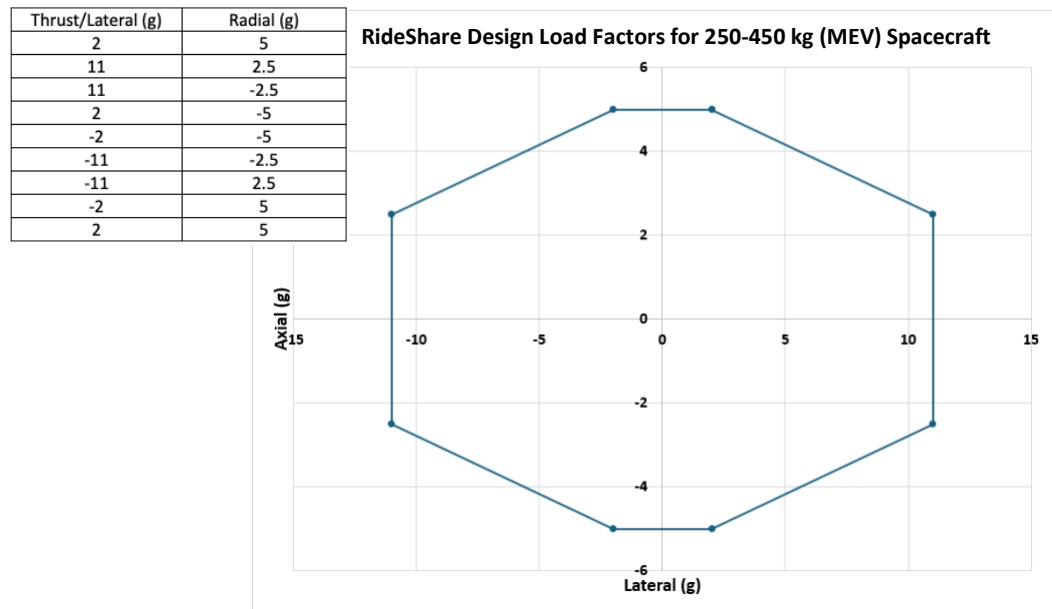
Figure 6.2 Side Mounted Design Load Factors (Updated in Rev 3)
